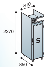
AGS 400
