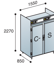
AGS 1300
